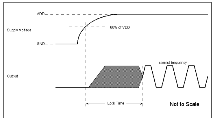
VCXO & FemtoClock PLL Lock Time
