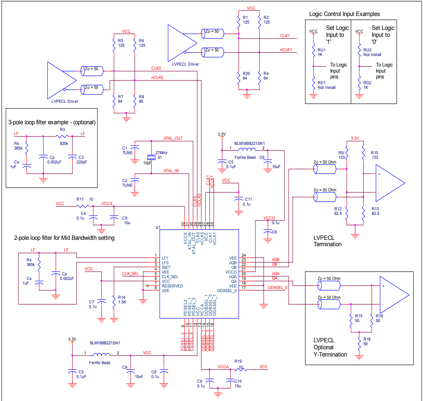
Figure 5. ICS813N252-02 Schematic Example
