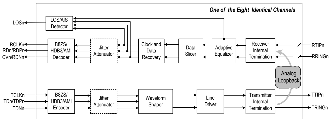
Figure-15 Analog Loopback
