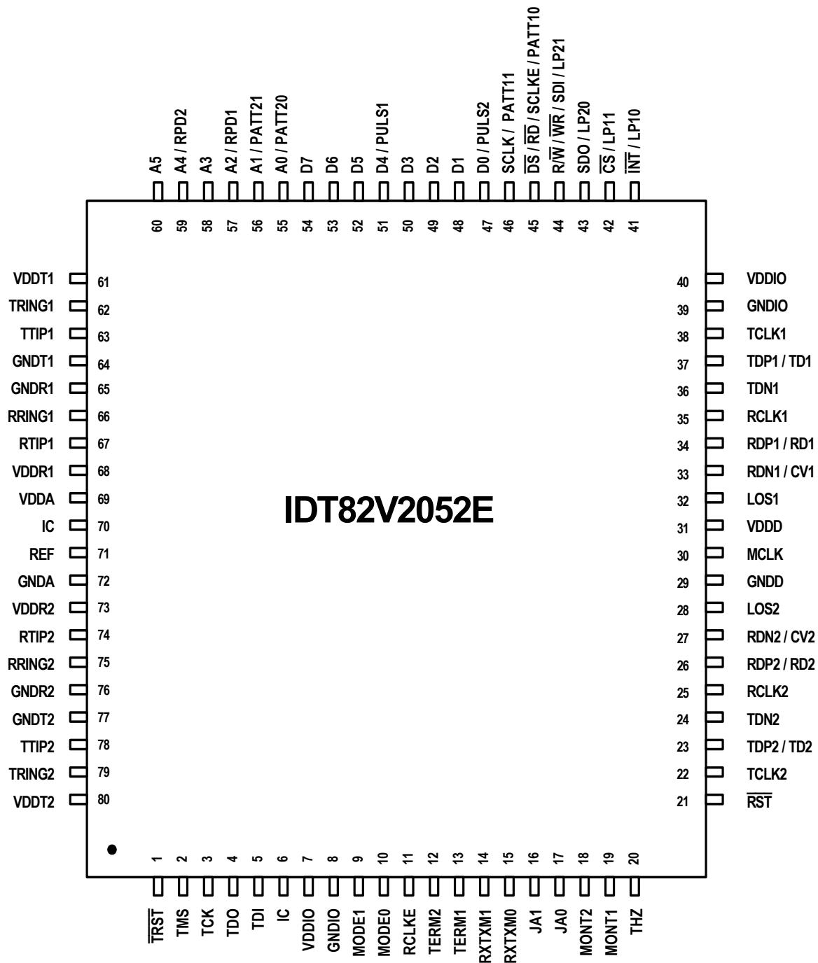
Figure-2 IDT82V2052E TQFP80 Package Pin Assignment
