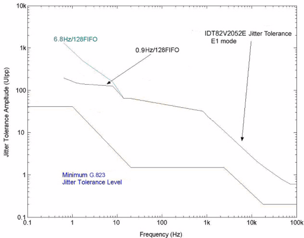
Figure-23 E1 Jitter Tolerance Performance
