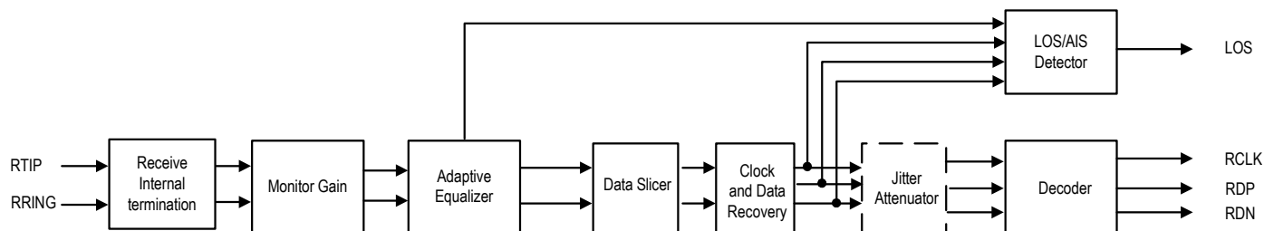
Figure-5 Receive Path Function Block Diagram
