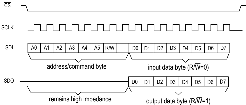
Figure-18 Serial Microcontroller Interface Function Timing
