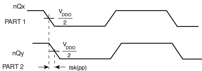
PART-TO-PART SKEW
