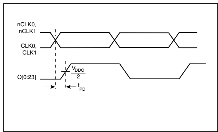
Propagation Delay
