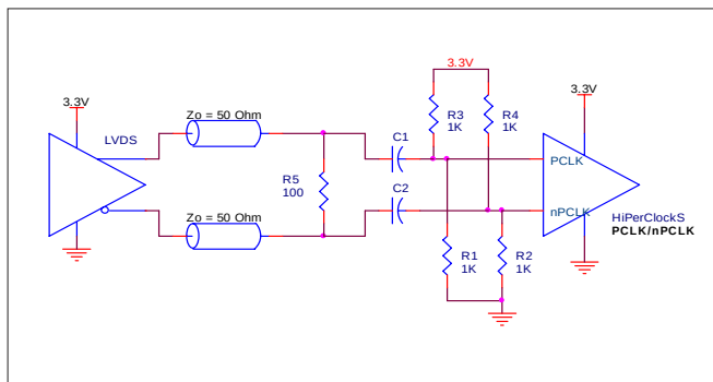
FIGURE 2D. PCLK/nPCLK INPUT DRIVEN BY A 3.3V LVDS DRIVER
