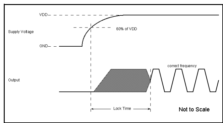
PLL Lock Time
