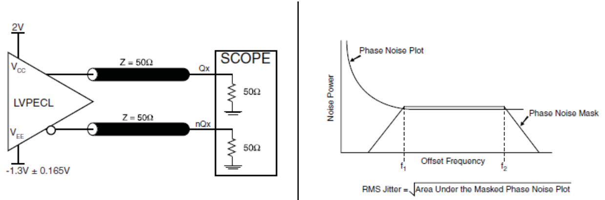
3.3V OUTPUT LOAD AC TEST CIRCUIT
