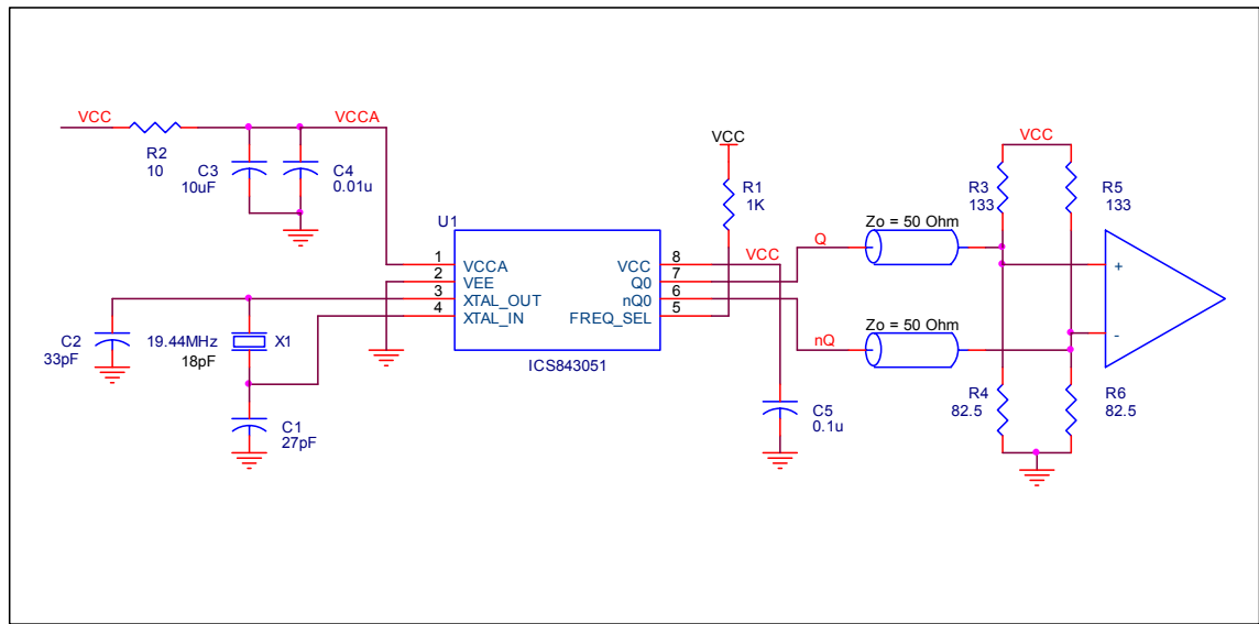
Figure 5A. ICS843051 Schematic Example
