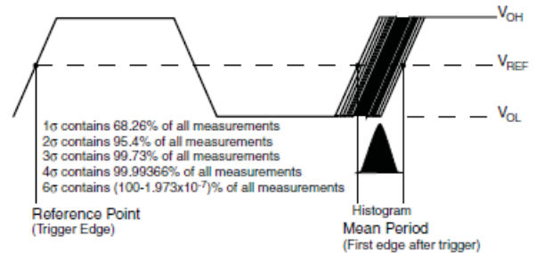
PERIOD JITTER
