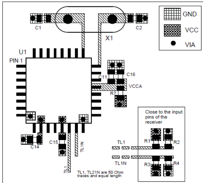
FIGURE 7B. PCB BOARD LAYOUT FOR 8430I-61
