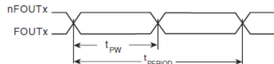
PERIOD JITTER
