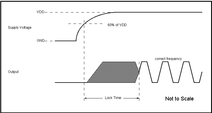
Lock Time
