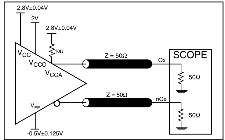
3.3V Core/ 2.5V LVPECL Output Load Test Circuit
