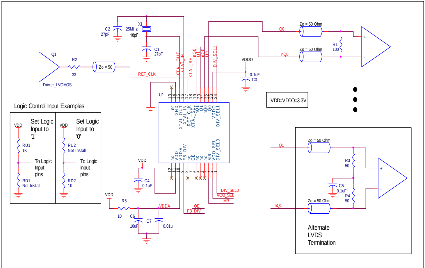
Figure 5. 844003EGI-01LF Schematic Layout Example
