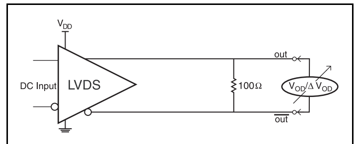
Differential Output Voltage Setup
