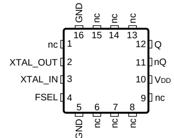
ICS844201I-45 16-Lead VFQFN Top View
