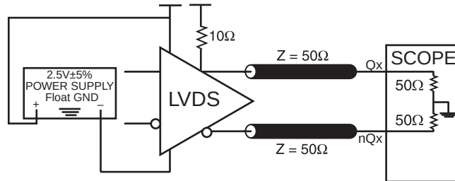
LVDS 2.5V OUTPUT LOAD AC TEST CIRCUIT
