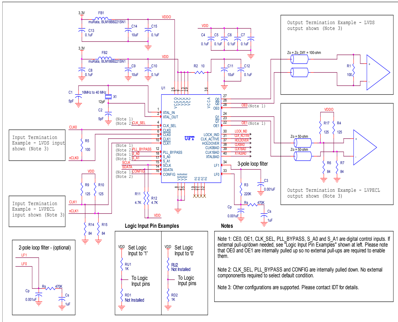
Figure 11. ICS849N202I Application Schematic
