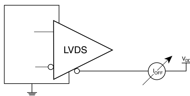
POWER OFF LEAKAGE SETUP
