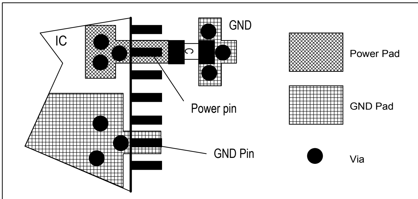
Figure 5B. Recommended Layout of Bypass Capacitor Placement
