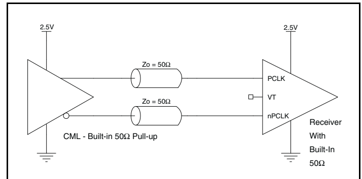
Figure 2D. PCLK/nPCLK Input with Built-In 50 \Omega Driven by a CML Driver with Built-In 50 \Omega Pullup
