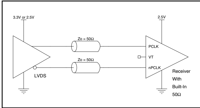
Figure 2A. PCLK/nPCLK Input with Built-In 50 \Omega Driven by an LVDS Driver
