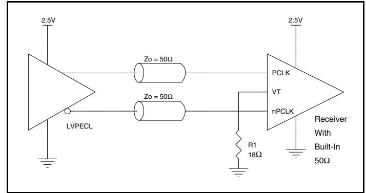
Figure 2B. PCLK/nPCLK Input with Built-In 50 \Omega Driven by an LVPECL Driver
