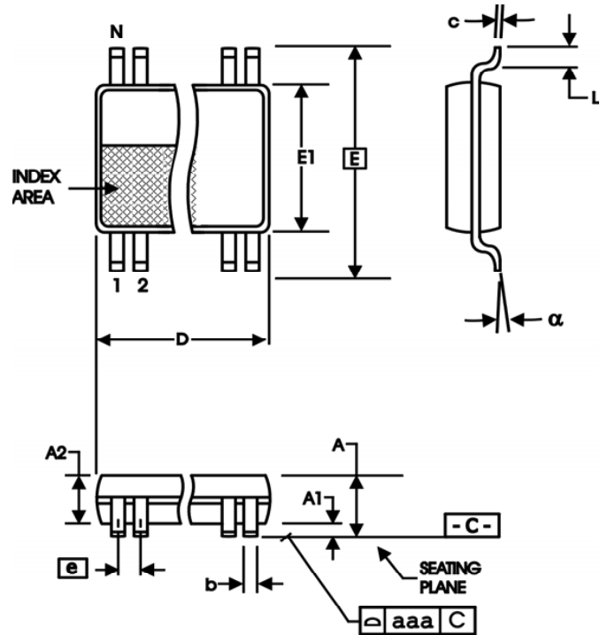
Package Outline - G Suffix for 20 Lead TSSOP
