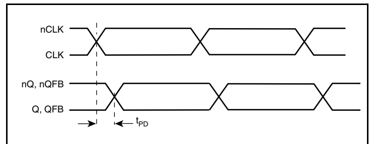
Propagation Delay
