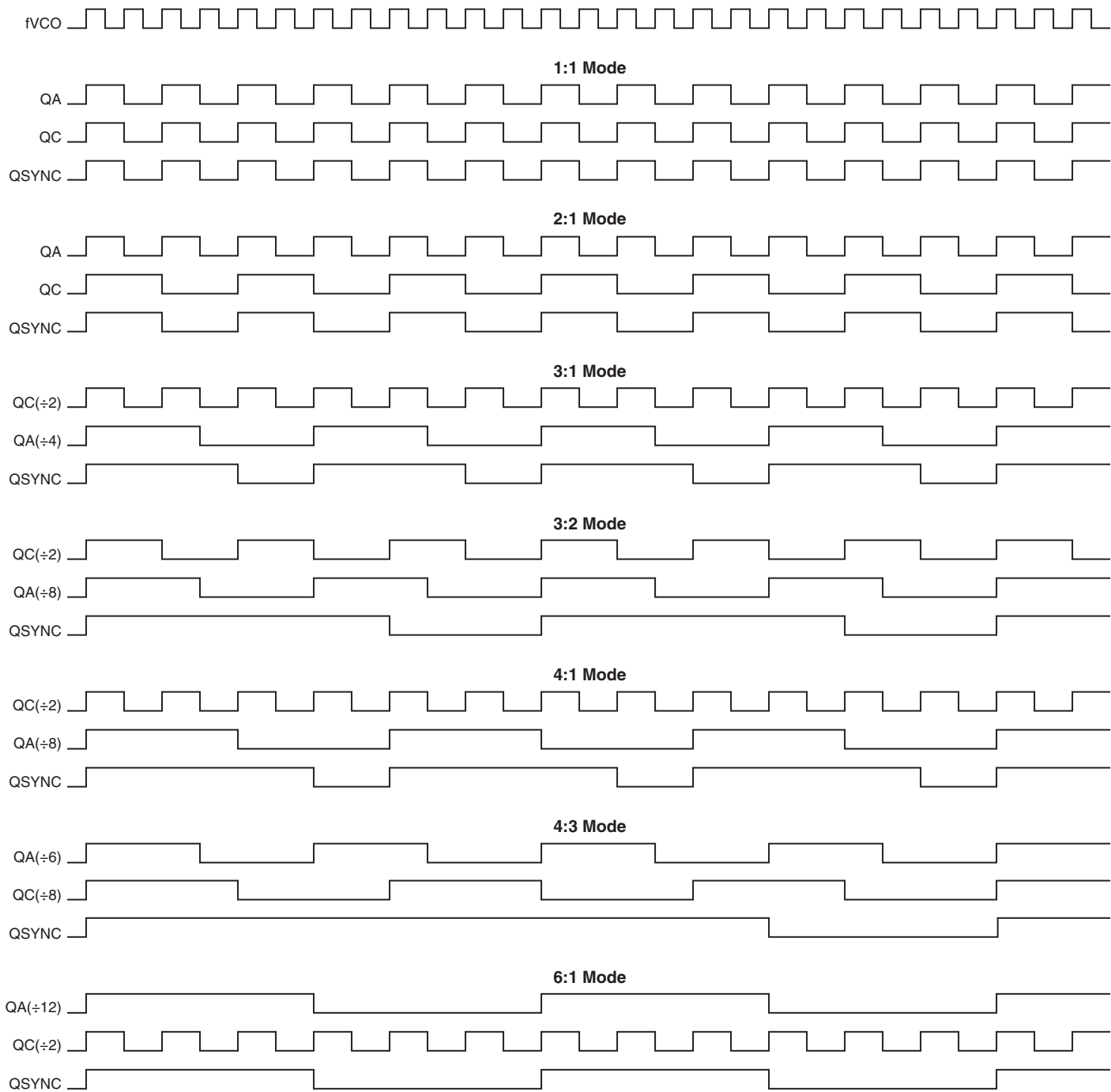
Figure 1. Timing Diagrams
