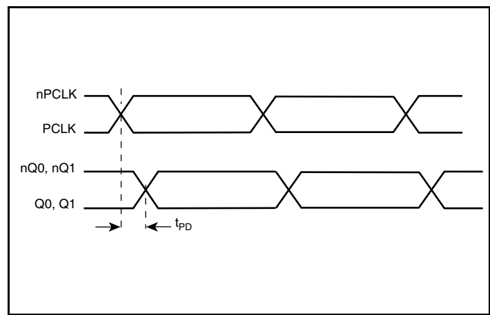
Propagation Delay
