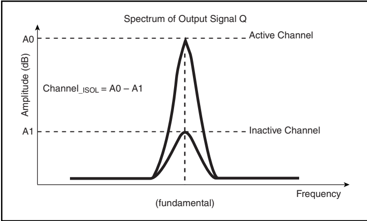
Channel Isolation
