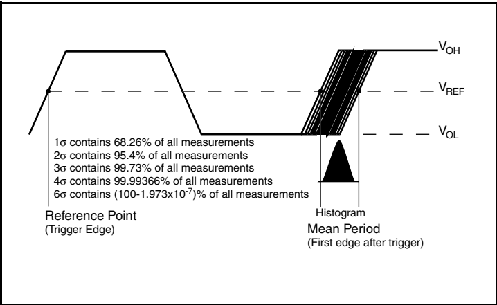
Period Jitter
