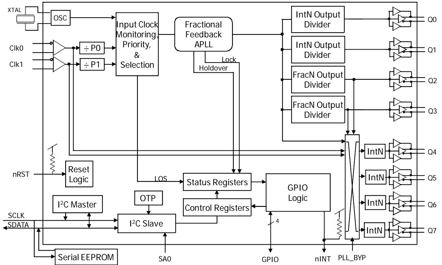
Figure 1: IDT8T49N281I Functional Block Diagram
