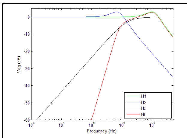
PCI Gen 1 Magnitude of Transfer Function
