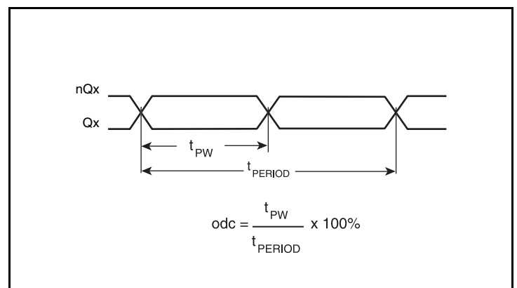
Differential Output Duty Cycle/Output Pulse Width/Period
