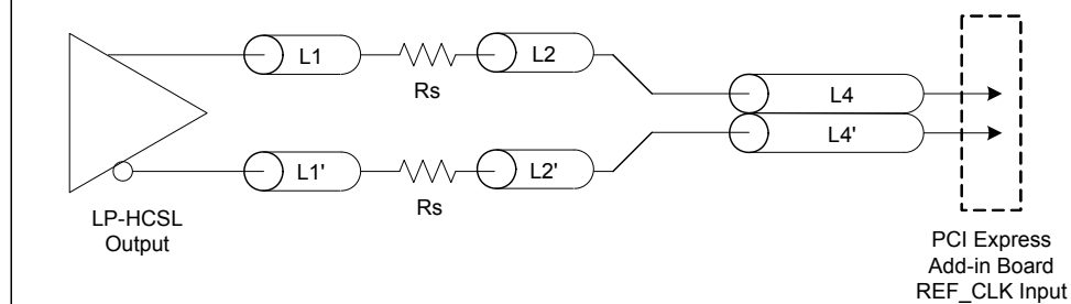
Figure 2: PCI Express Connector Routing
