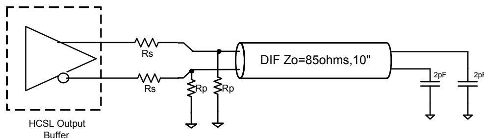
9ZX21200 Differential Test Loads
