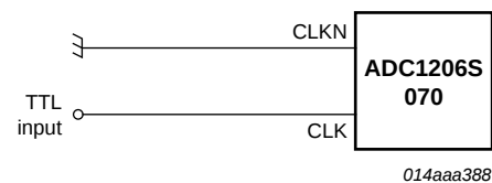
Fig 19. Application diagram for TTL single-ended clock
