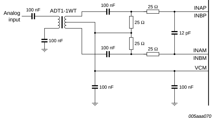
Fig 8. Single transformer configuration
