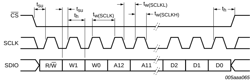
Fig 5. SPI timing
