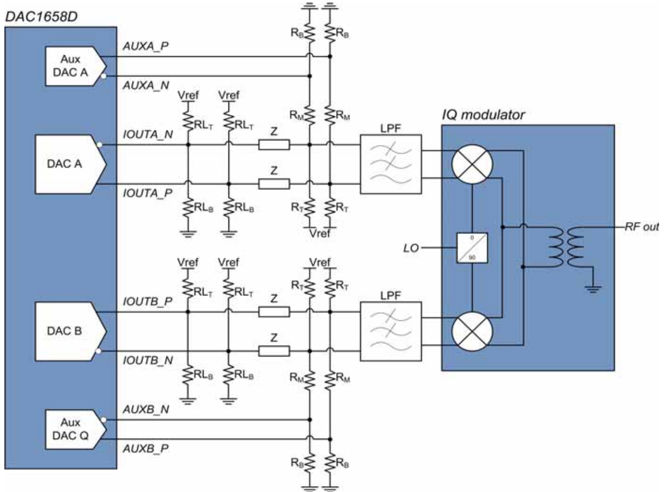
Fig 84. 1 V (p-p) interface to IQ-modulator (High common mode version)
