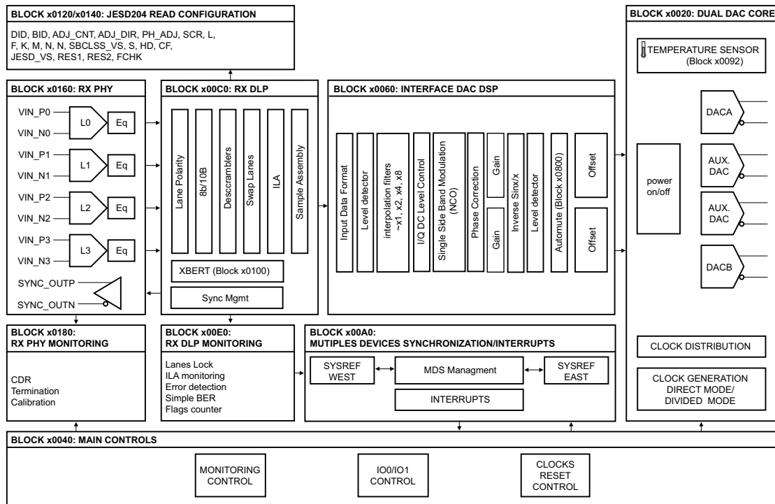
Fig 33. SPI register blocks partition
