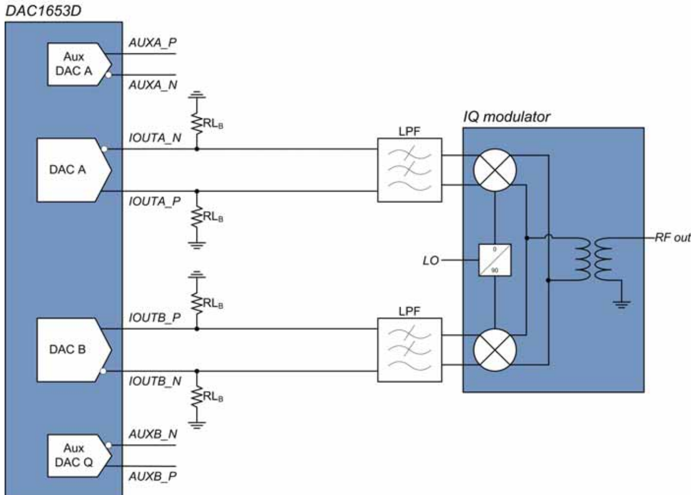
Fig 85. 1 V (p-p) interface to IQ-Modulator (Low common mode version)
