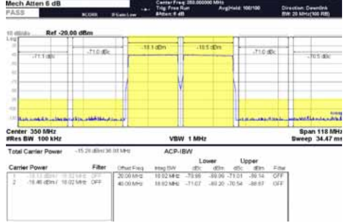
Fig 22. ACLR of 2 carriers LTE (BW=2 x 20 MHz) centered at 350 MHz
