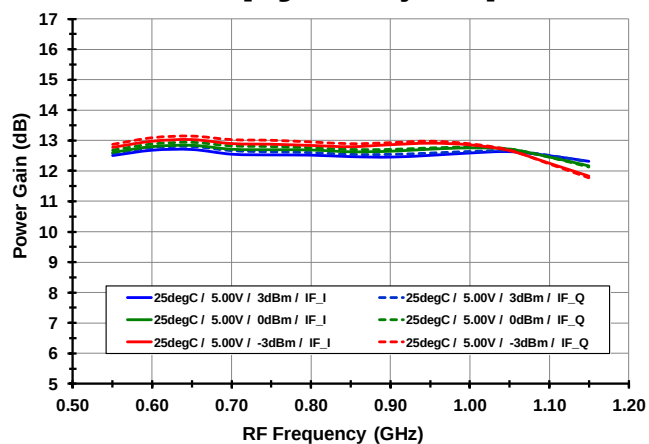
GAIN vs. LO level [High Side Injection]
