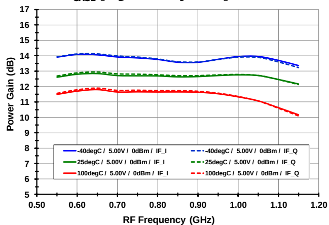
GAIN vs. T_{CASE} [High Side Injection]
