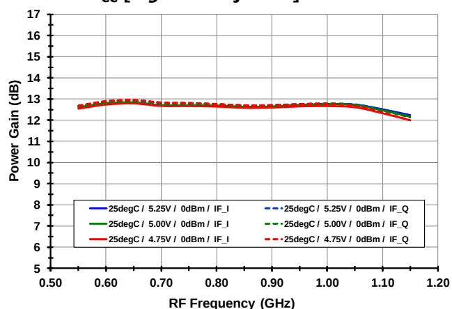
GAIN vs. V_{CC} [High Side Injection]
