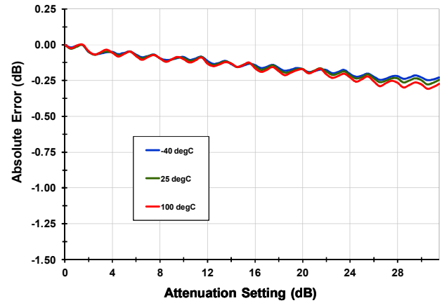
INL [1900 MHz]
