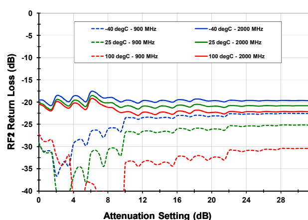
S_{22} vs. Attenuation State
