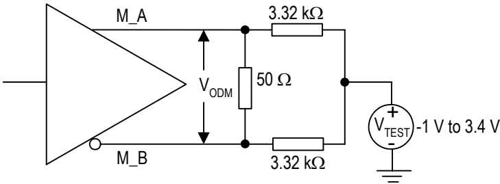
Figure-15 M-LVDS Output Voltage Test Circuit
