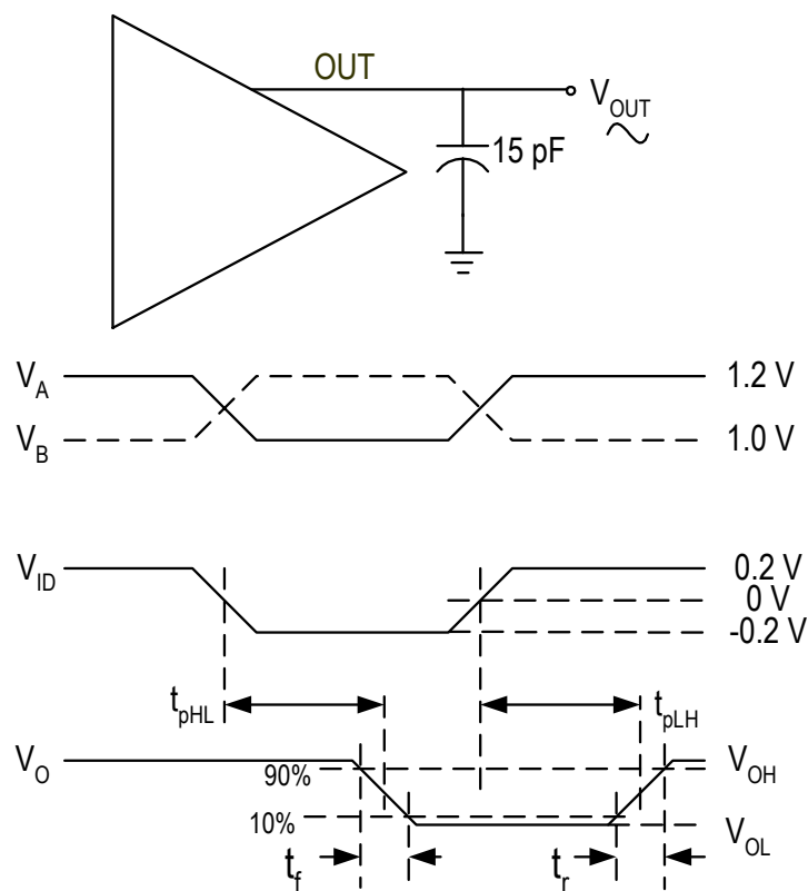
Figure-3 LVTTL Output Test Circuit and Waveforms
