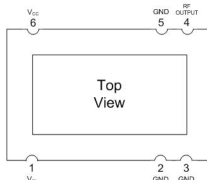
Figure 1: Pin Assignment
