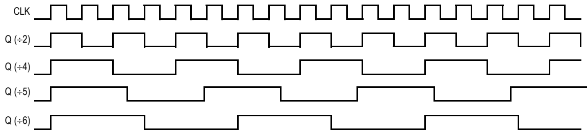
Figure 3. Timing Diagram
