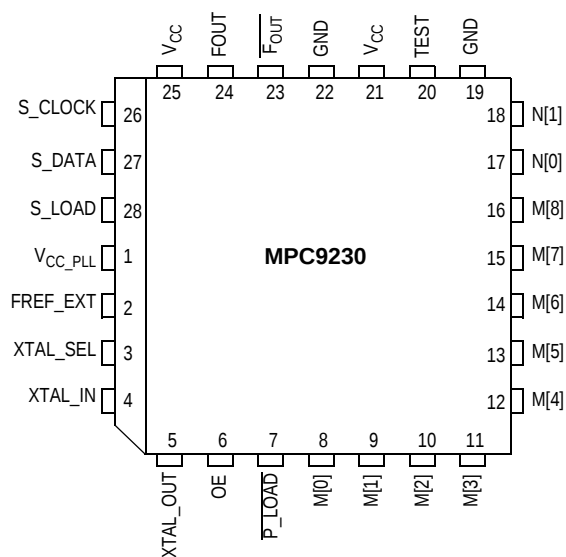
Figure 2. MPC9230 28-Lead PLCC Pinout (Top View)
