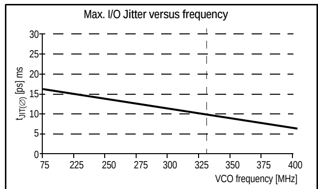
Figure 5. Max. I/O Jitter (RMS) Versus Frequency for V_{CC} = 3.3\text{ V}
