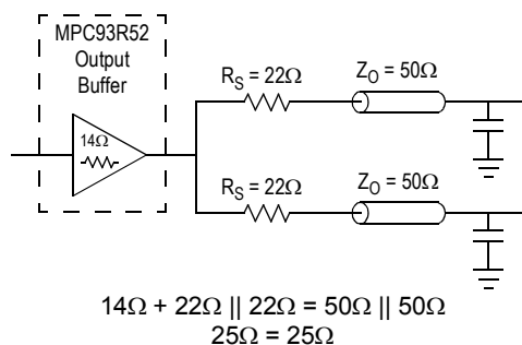
Figure 12. Optimized Dual Line Termination
