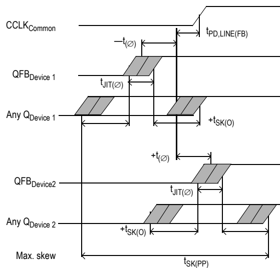
Figure 8. MPC93R52 Max. Device-to-Device Skew
