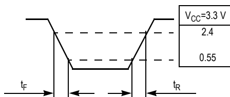
Figure 20. Output Transition Time Test Reference
