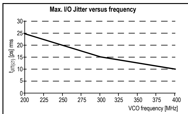
Figure 9. Max. I/O Jitter versus Frequency
