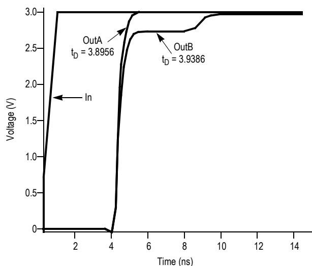
Figure 11. Single versus Dual Waveforms
