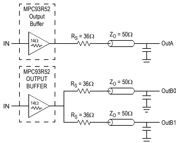
Figure 10. Single versus Dual Transmission Lines
