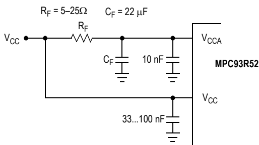
Figure 7. V_{CCA} Power Supply Filter
