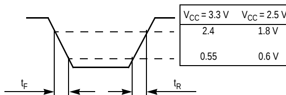
Figure 13. Output Transition Time Test Reference
