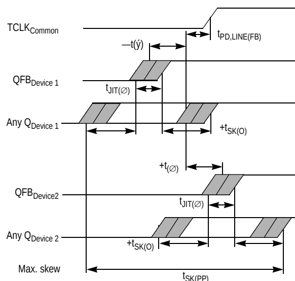
Figure 7. MPC961P Max. Device-to-Device Skew
