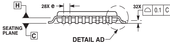
DETAIL AD
