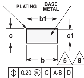
SECTION F-F
