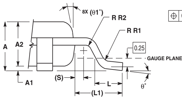
DETAIL AD
