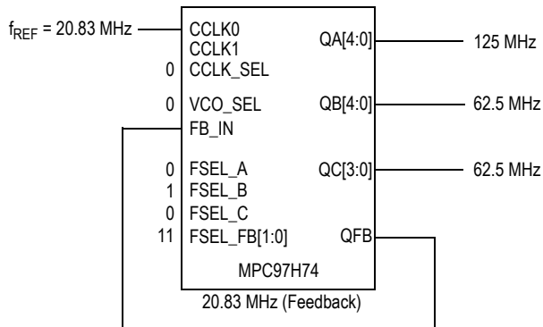
MPC97H74 example configuration (feedback of QFB = 20.83 MHz, VCO_SEL = \div 2 , M = 12 , N_A = 2 , N_B = 4 , N_C = 4 , f_{VCO} = 500 MHz). T_A = 0^\circ\text{C} to 70^\circ\text{C}
