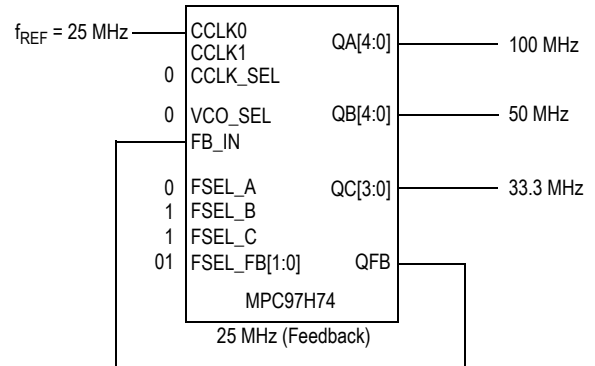
MPC97H74 example configuration (feedback of QFB = 25 MHz, VCO_SEL = \div 2 , M = 8 , N_A = 2 , N_B = 4 , N_C = 6 , f_{VCO} = 400 MHz).
