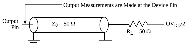
Figure 13. AC Test Load for the Tsi107
