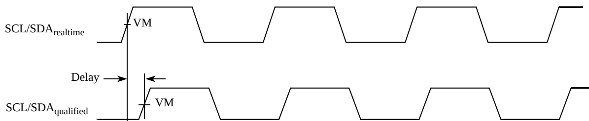
Figure 18. I 2 C Timing Diagram IV (Qualified Signal)
