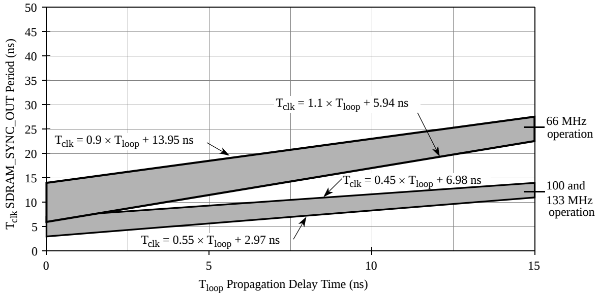
Figure 8. DLL Locking Range Loop Delay ( DLL\_STANDARD = 0 )
