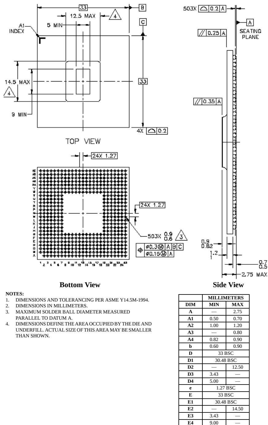
Figure 25. Tsi107 Package Dimensions and Pinout Assignments
