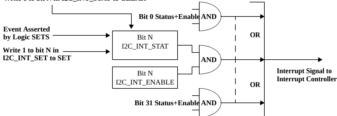
Figure 43: I 2 C Interrupt Generation
