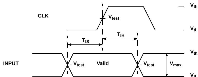
Figure 52: Input Timing Measurement Waveforms
