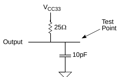
Figure 55: PCI T_{OV(max)} Falling Edge AC Test Load
