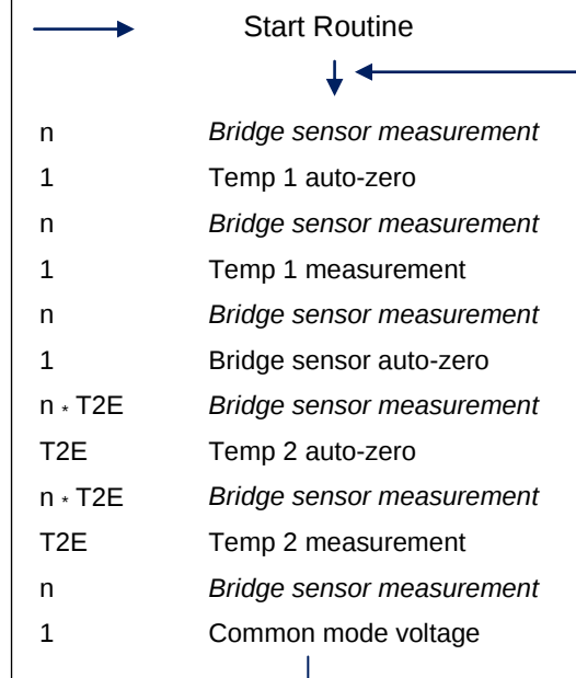
Figure 2.2. Measurement Cycle ZSC31050
