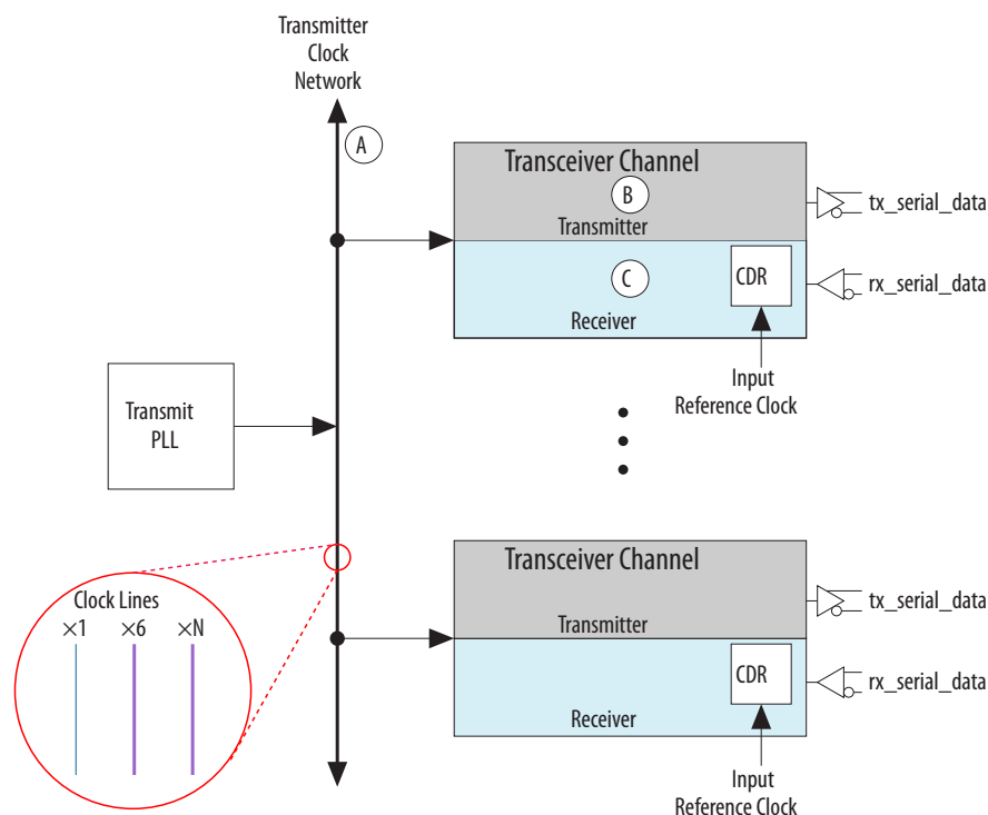
Figure 2-7: Internal Clocking
