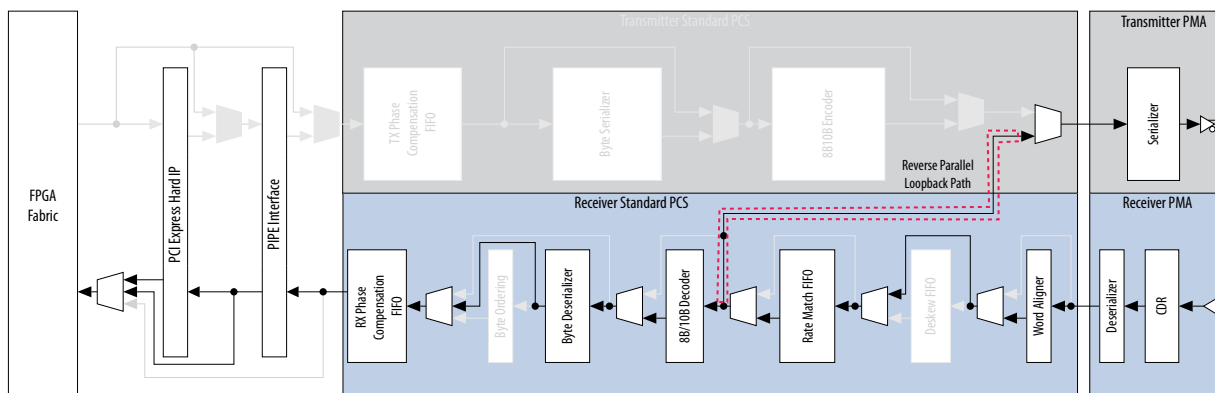
Figure 4-20: PCIe Reverse Parallel Loopback Mode Datapath
