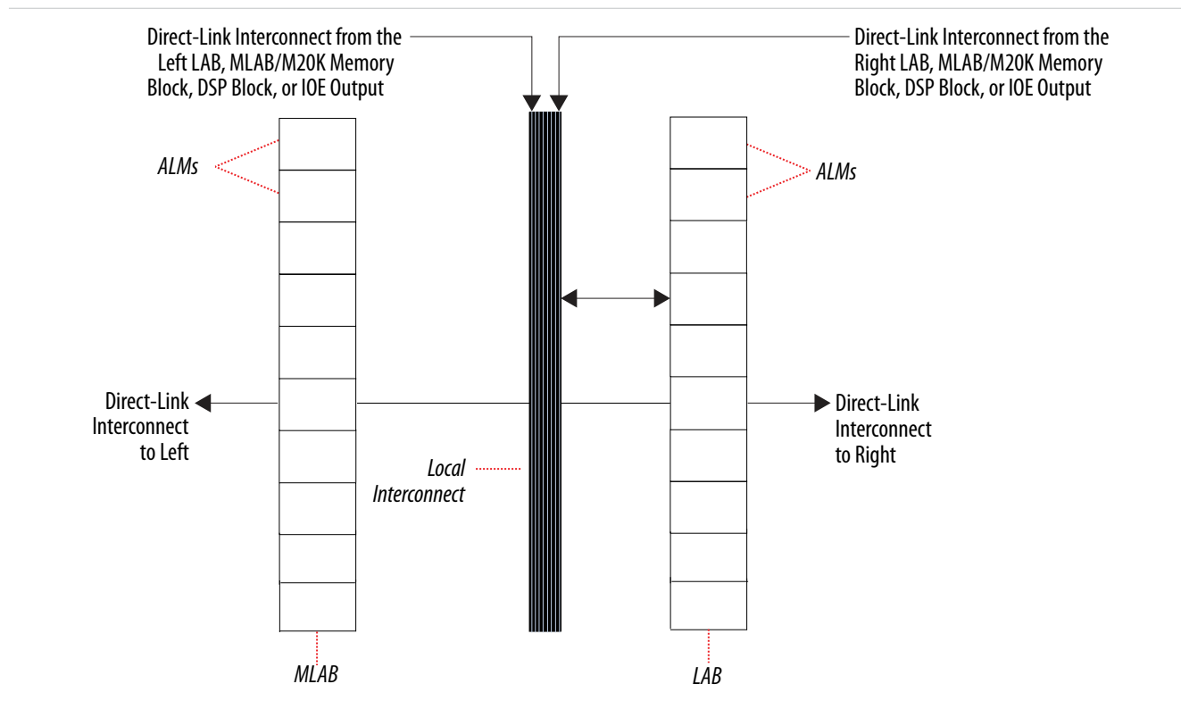
Figure 1-3: LAB Fast Local and Direct Link Interconnects for Stratix V Devices
