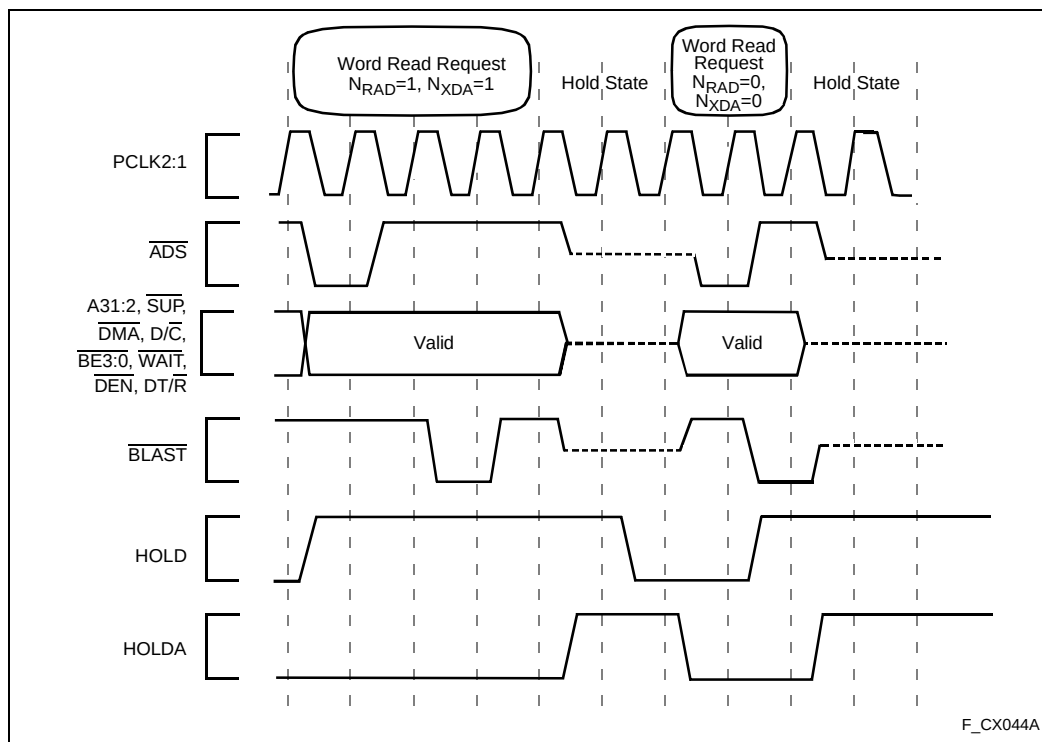
Figure 42. HOLD Functional Timing
