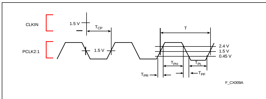
Figure 9. CLKIN Waveform
