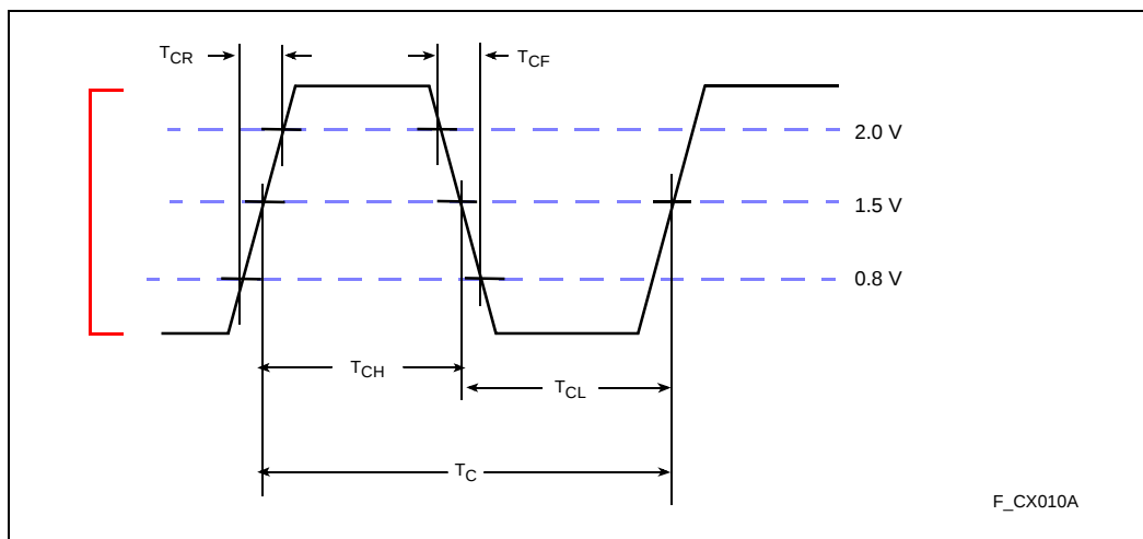
Figure 9. CLKIN Waveform
